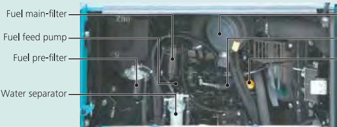
Large rear maintenance space
